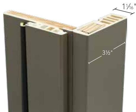
3 1/2" FLAT RIPPABLE BRICKMOLD
